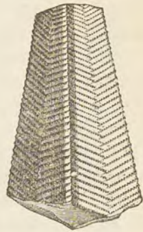
CONULARIA ORNATA. (Old Red Sandstone.)
